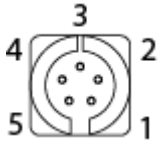
Male connector on SPY RF U
